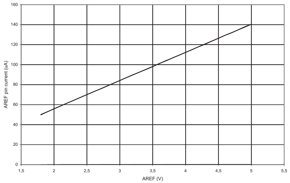
Figure 21-127. AREF Pin Current vs. Pin Voltage
