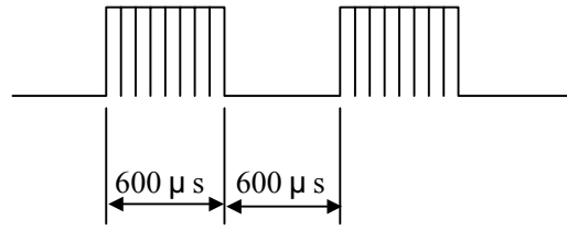
fig. 1 Transmit signal
