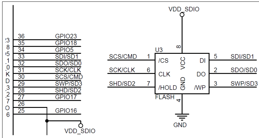
Figure 6: ESP32 Flash
