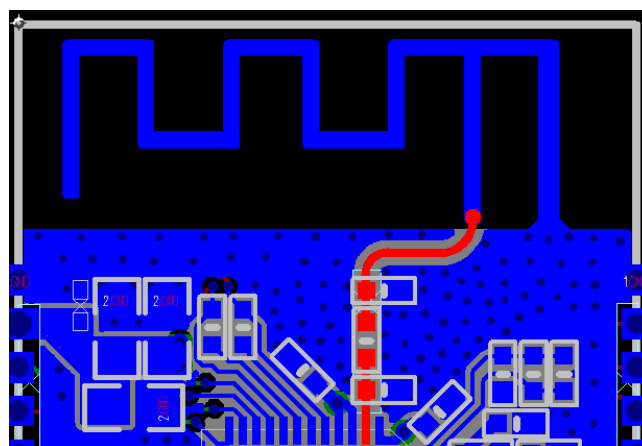
Figure 14: ESP32 RF
