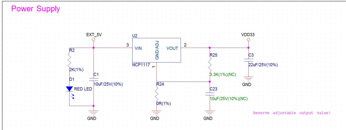
Figure 20: Power Schematics of ESP32-DevKitC
