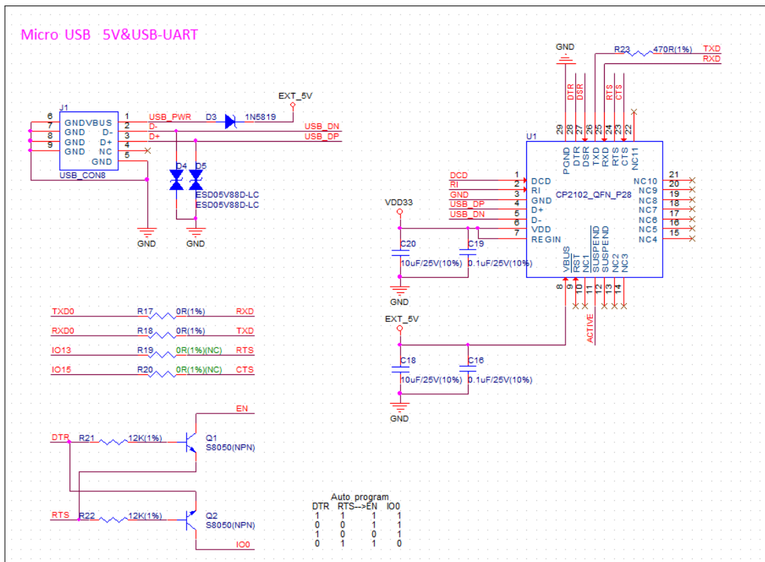
Figure 21: USB-UART Schematics
